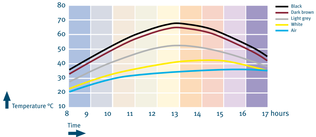
Temperature curve of PVC-U sheet surfaces at a maximum air temperature of 36 °C
