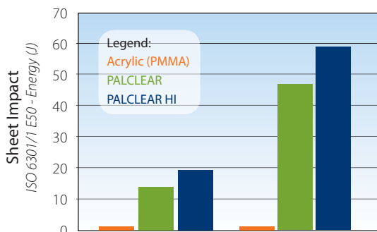
Impact Resistance Comparison at 23°C
